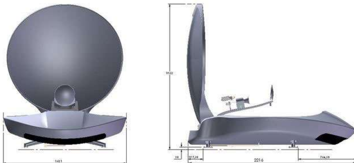
Front and side view of PDA-150 DriveNews™
